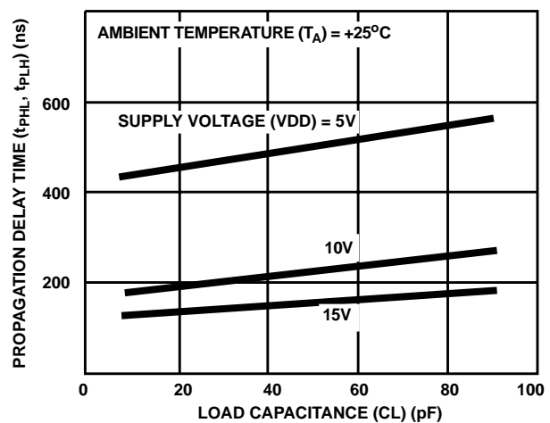
FIGURE 9. TYP. PROPAGATION DELAY TIME AS A FUNCTION OF LOAD CAPACITANCE (+ OR - TRIGGER TO Q, \bar{Q} )
