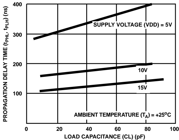
FIGURE 8. TYP. PROPAGATION DELAY TIME AS A FUNCTION OF LOAD CAPACITANCE (ASTABLE, ASTABLE TO Q, \bar{Q} )
